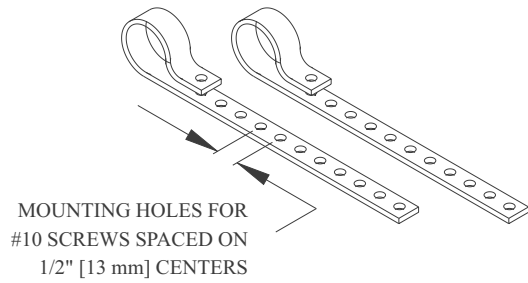
STANDARD MOUNTING BRACKETS
